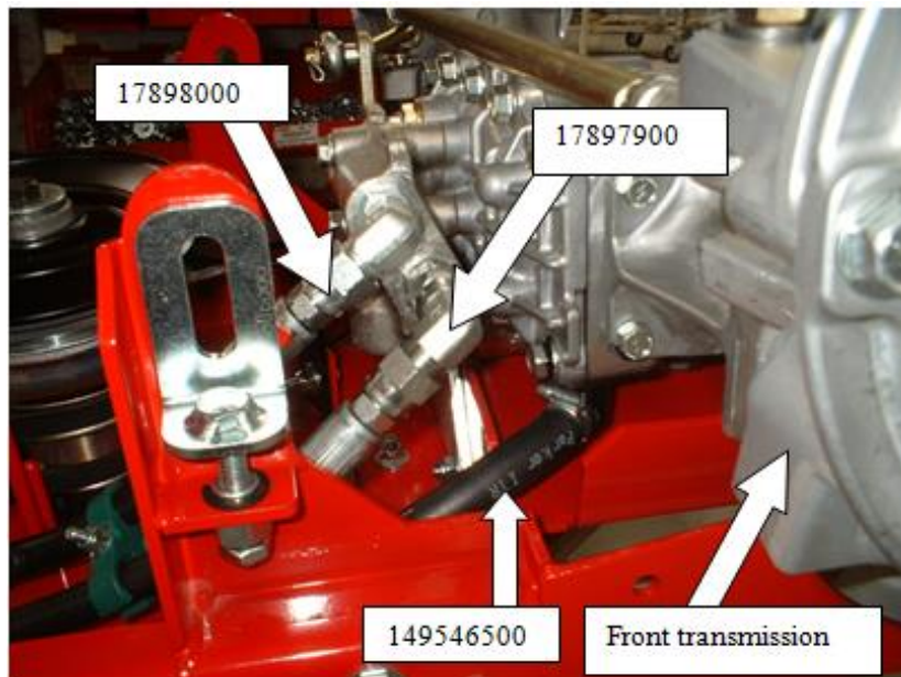
Figure 1: Front transmission pipes
