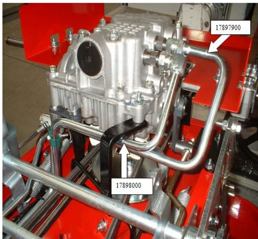
Figure 4: Rear Transmission
