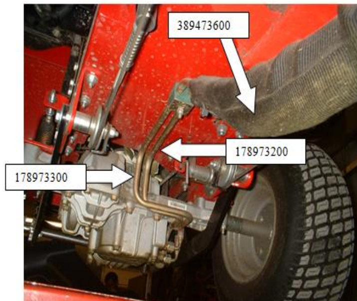
Figure 3: Front transmission pipes. View from underneath tractor
