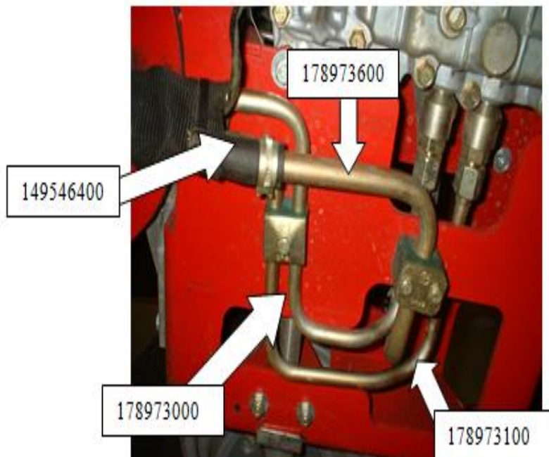
Figure 2: Rear Bogey transmission pipes View from underneath tractor
