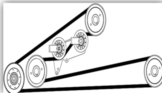
50" Combi
