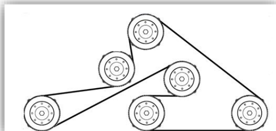
50" Mulcher
