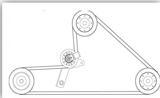
38" & 44" Combi & Mulcher
